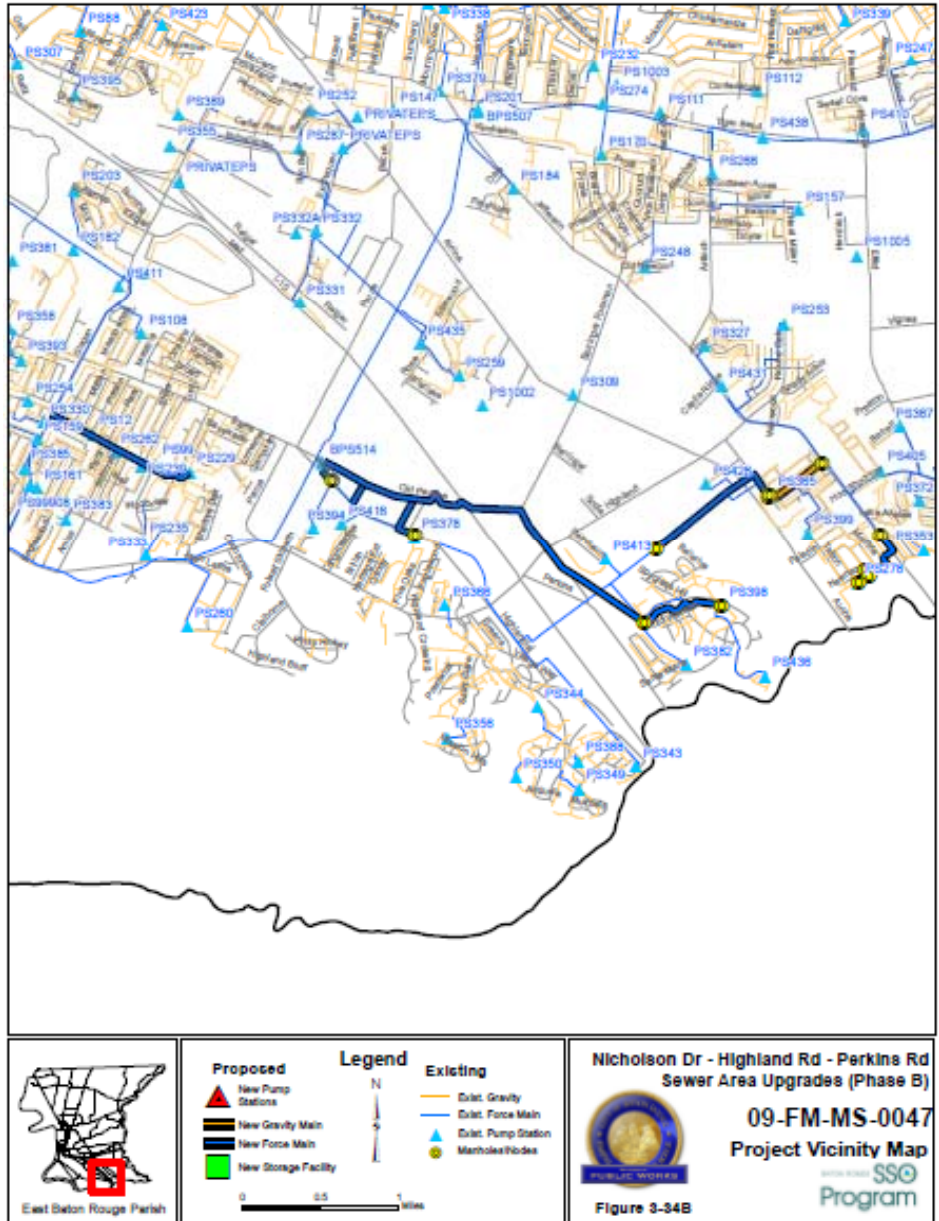
Flow measurements are taken throughout the collection system to determine the correct pump station upgrade size.
